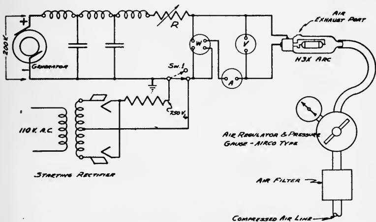
FIG. 5. Control circuit of air-cooled H3X arc.
